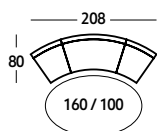
Oval 160 (3 parts)
